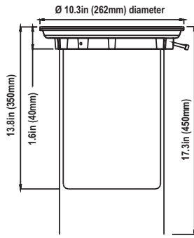
LS640-K SECTION
