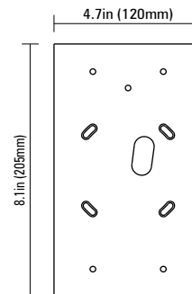
LS6050 Mounting Plate 4in J-Box
