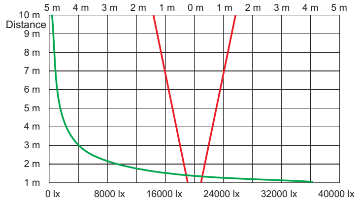
Beam Dimensions
