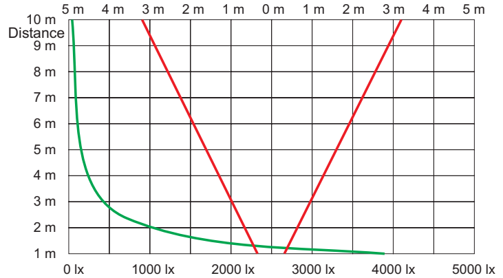
Beam Dimensions
